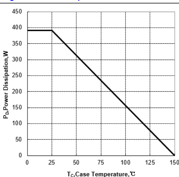
Figure 2 Power Dissipation
